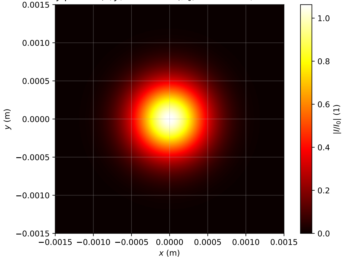
Intensity profile I(x, y, z = 0.478m)/I_0 , P_{in}=0.6P_{cr} , artificial time
